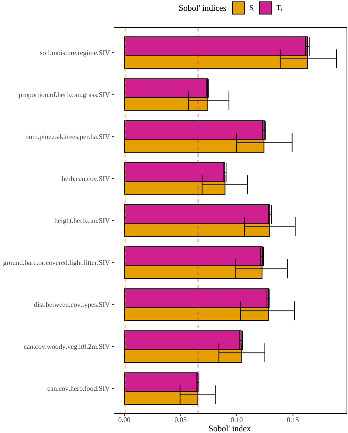
Figure 4. Results of a sensitivity analysis for the northernbobwhiteDbh27.9cm model based on an arithmetic mean structure. Dashed lines represent baseline numerical approximation error for S_i and T_i ( i.e. , dummy variables).
